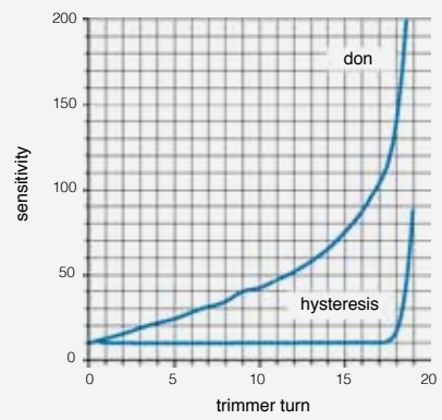
sensitivity adjustment
